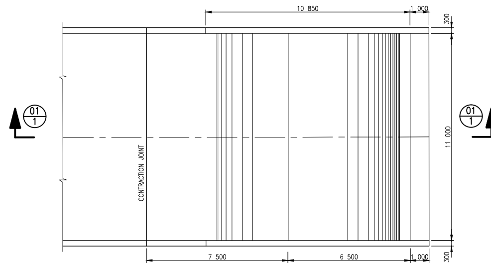
PLAN OF FLIP BUCKET SCALE 1 : 200
